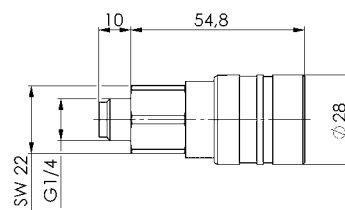
Order no. 427872 Sleeve
