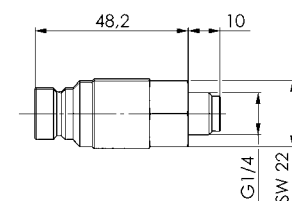
Order no. 427856 Connector
